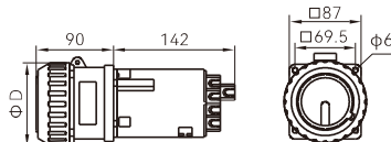
Socket without enclosure (M)
