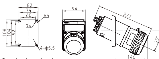
Opening hole drawing
