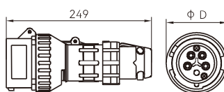
Plug (T)
